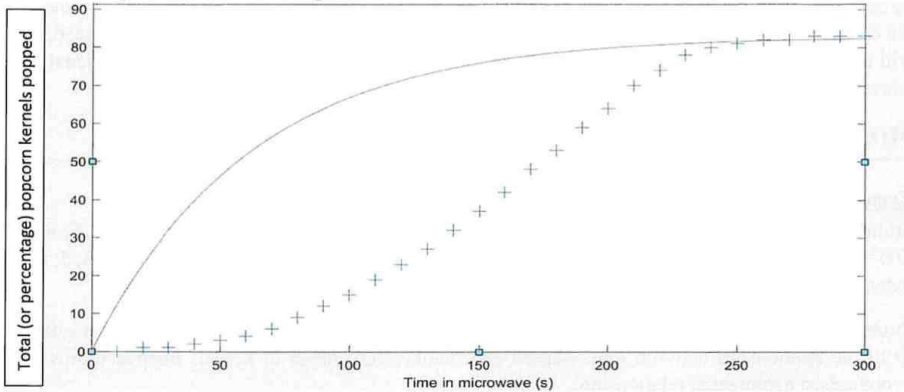
Fig. 3 Exponential model (orange) compared to cumulative frequency plot (blue)
