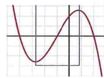
Fig. 4 General cubic function with negative leading coefficient image from Wikipedia
