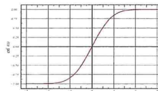
Fig. 7 Graph of the error function, erf(x), image from Wikipedia
