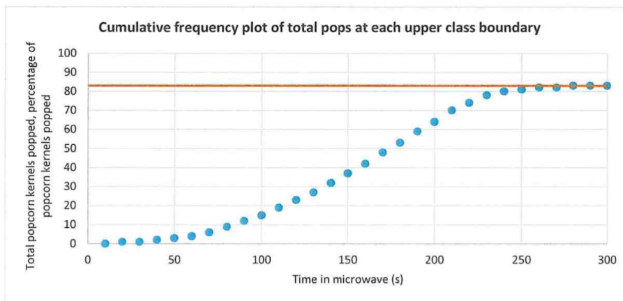
Fig. 2 Cumulative frequency plot of the number pops (blue) with a horizontal asymptote of y = 83 (orange)
